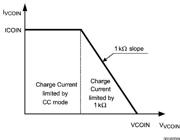
FIGURE 2. BBC IU Characteristic
