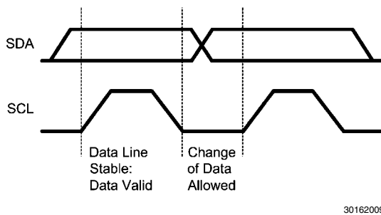
FIGURE 3. Bit Transfer
