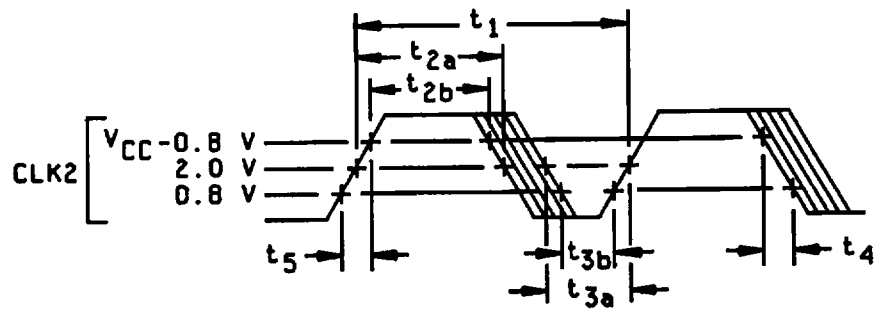
CLK2 TIMING
