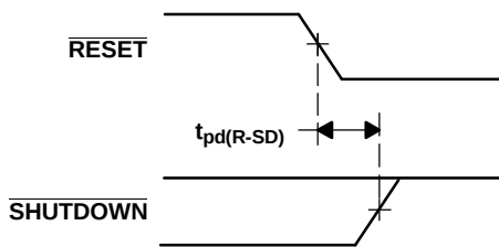
Figure 2. \overline{\text{RESET}} to \overline{\text{SHUTDOWN}} Propagation Delay
