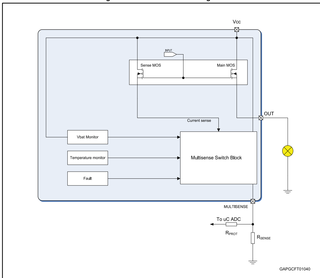
Figure 33: MultiSense block diagram
