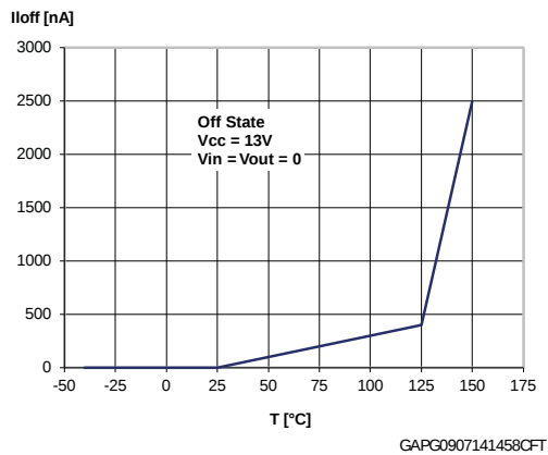
Figure 10: OFF-state output current
