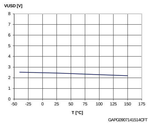
Figure 19: Undervoltage shutdown
