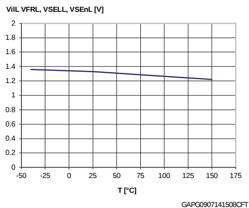
Figure 14: Logic Input low level voltage
