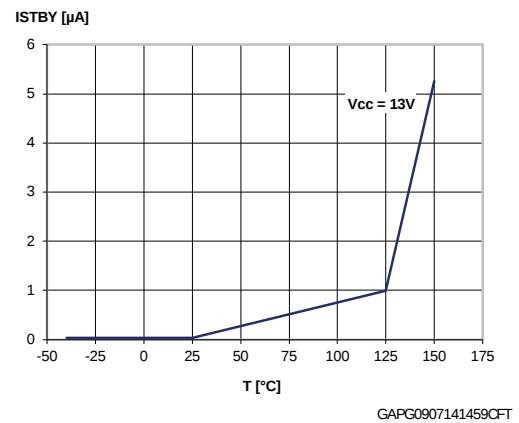
Figure 11: Standby current
