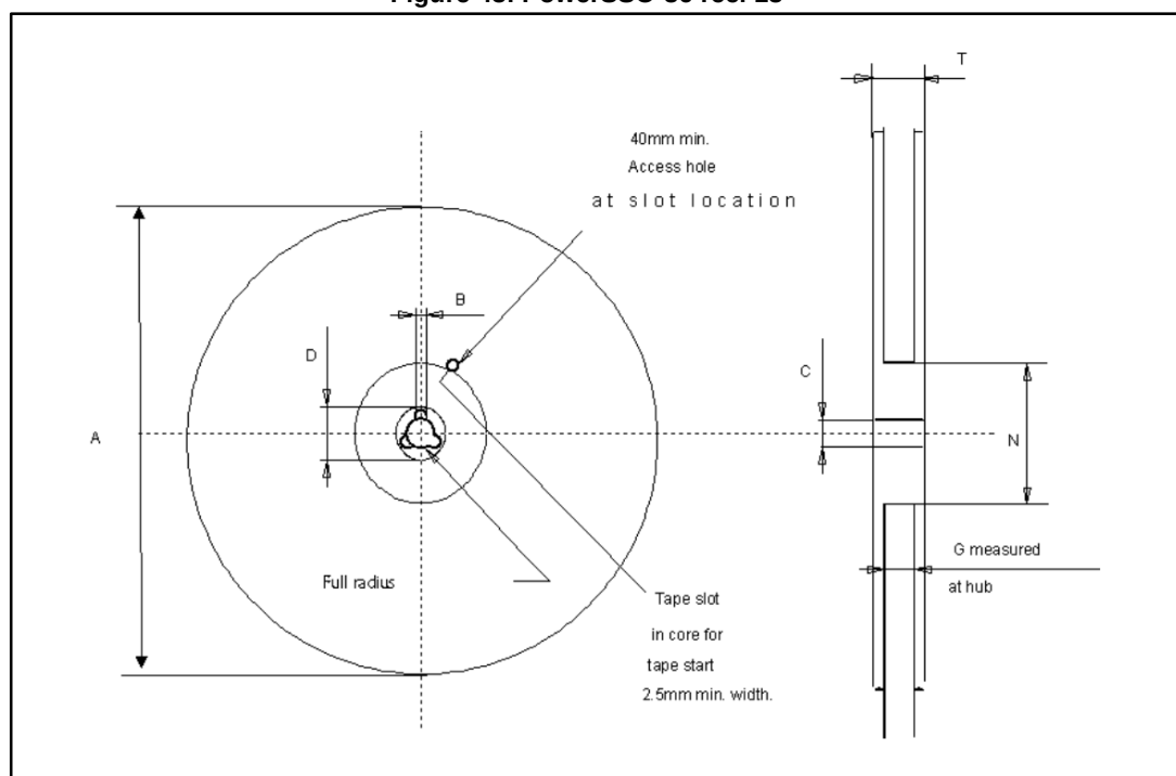
Figure 43: PowerSSO-36 reel 13"
