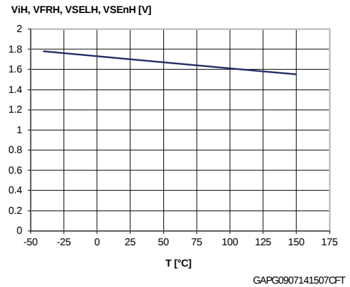
Figure 13: Logic Input high level voltage
