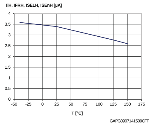
Figure 15: High level logic input current
