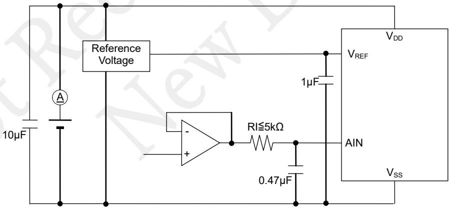
Measuring circuit
