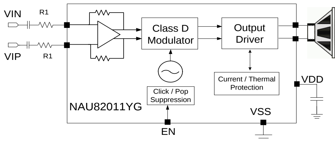
Figure 1: NAU82011YG Block Diagram
