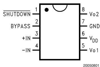
Top View Order Number LM4905MM See NS Package Number MUA08A
