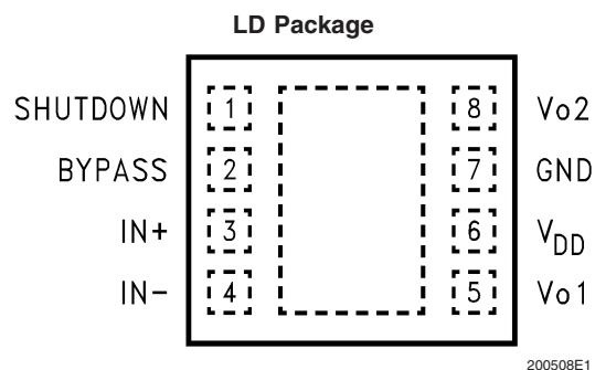
Top View Order Number LM4905LD See NS Package Number LDA08A
