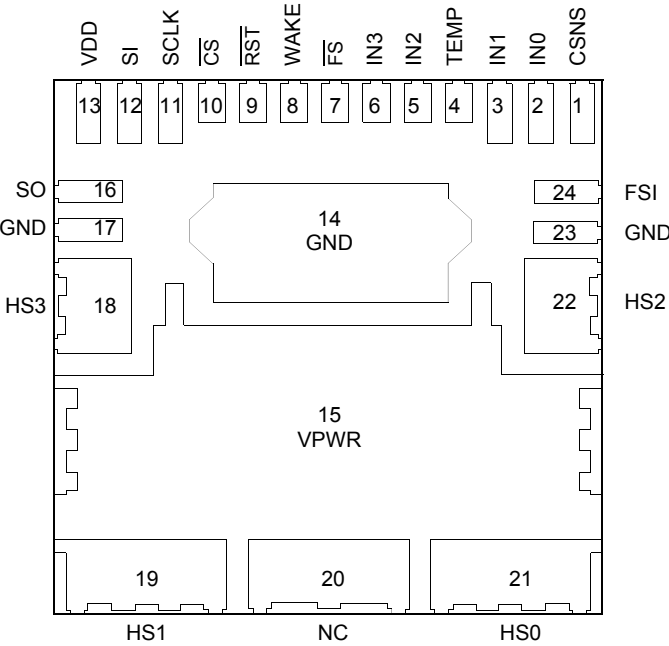
Figure 3. 33874 Pin Connections
