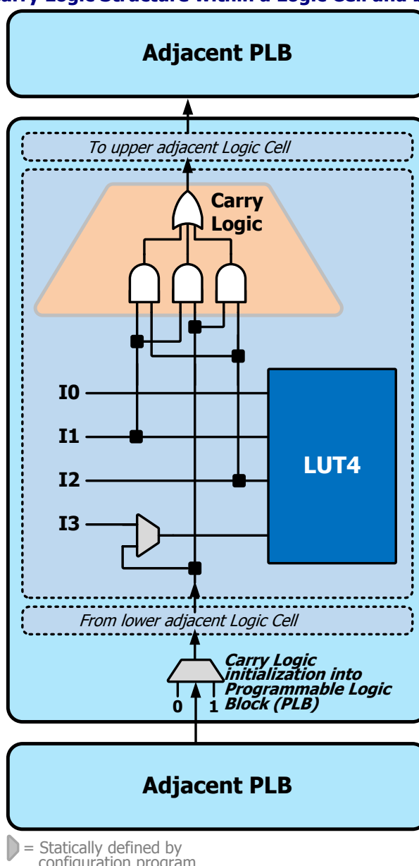
Figure 4: Carry Logic Structure within a Logic Cell and between PLBs
