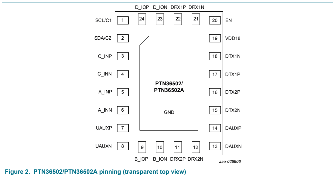
Figure 2. PTN36502/PTN36502A pinning (transparent top view)
