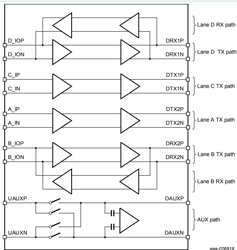
Figure 9. Different lane TX and RX paths definitions
