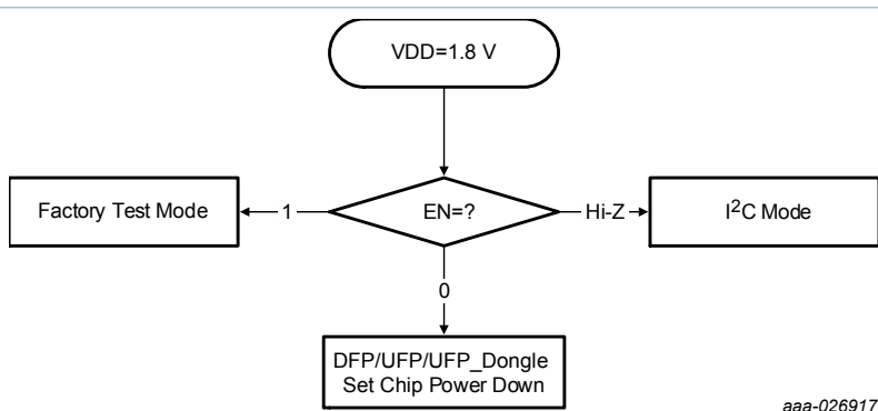
Figure 8. EN control flow diagram
