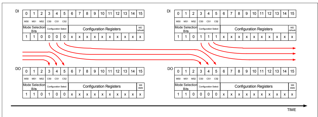
Figure 34 Write Command
