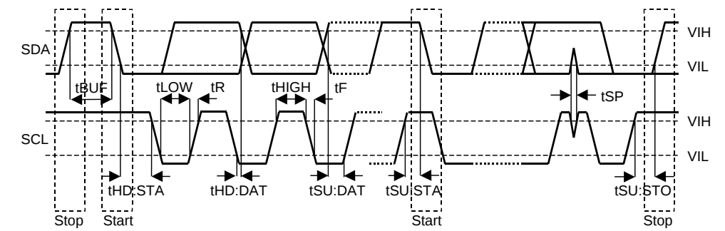
Figure 9. I 2 C Bus mode Timing
