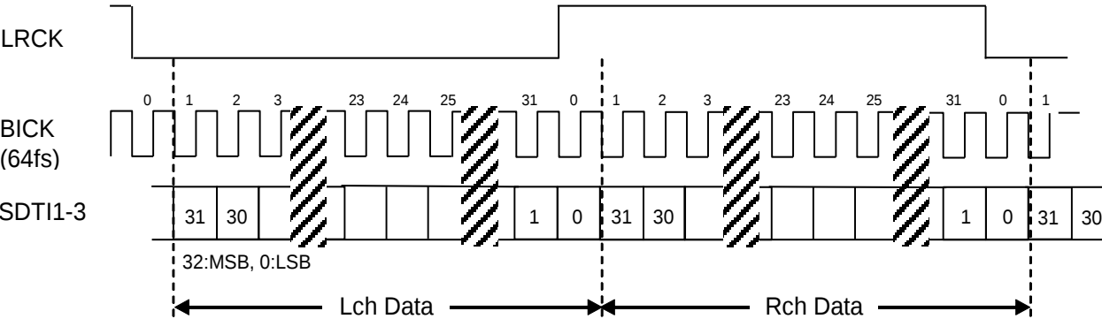
Figure 16. Mode 7 Timing
