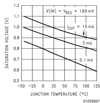
Output Saturation Voltage ( V_{SAT} )
