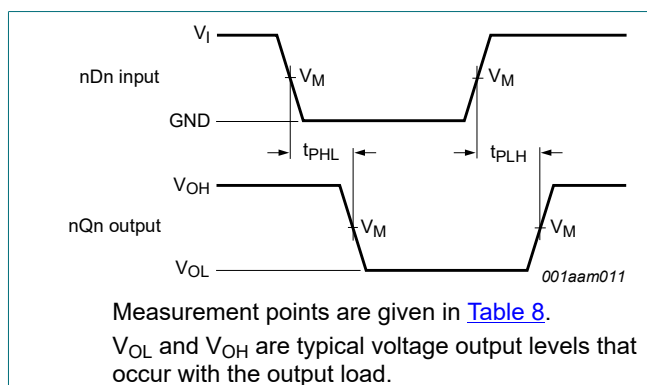
Fig. 5. Input (nDn) to output (nQn) propagation delays
