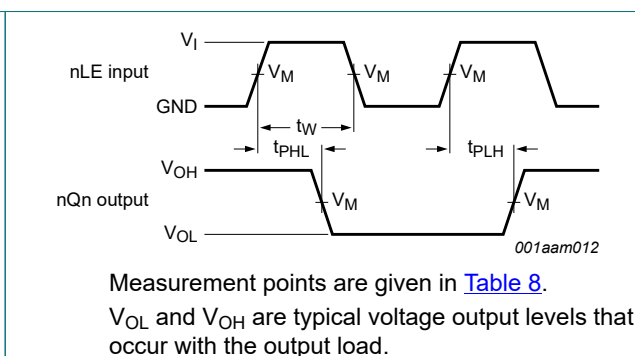
Fig. 6. Latch enable input (nLE) to data output (nQn) propagation delays and pulse width
