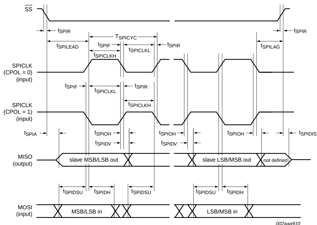
Fig 28. SPI slave timing (CPHA = 0)
