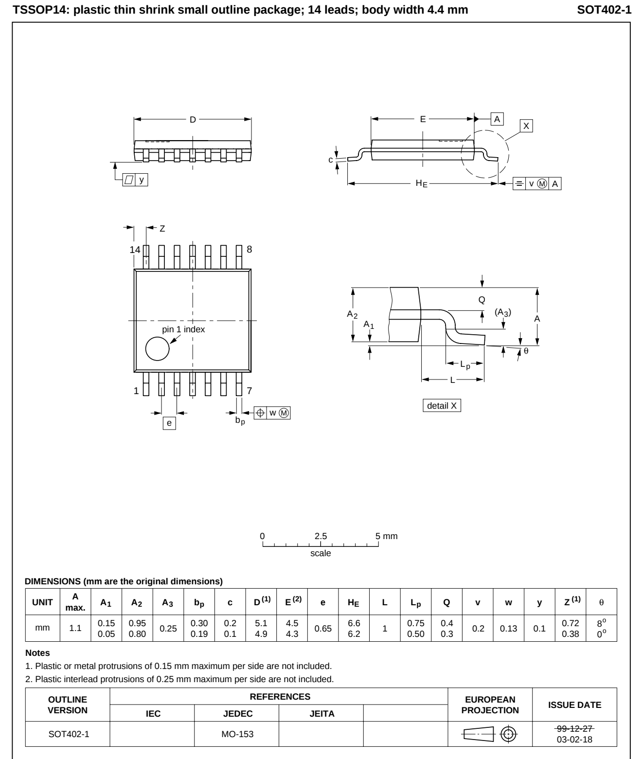
Fig 30. Package outline SOT402-1 (TSSOP14)
