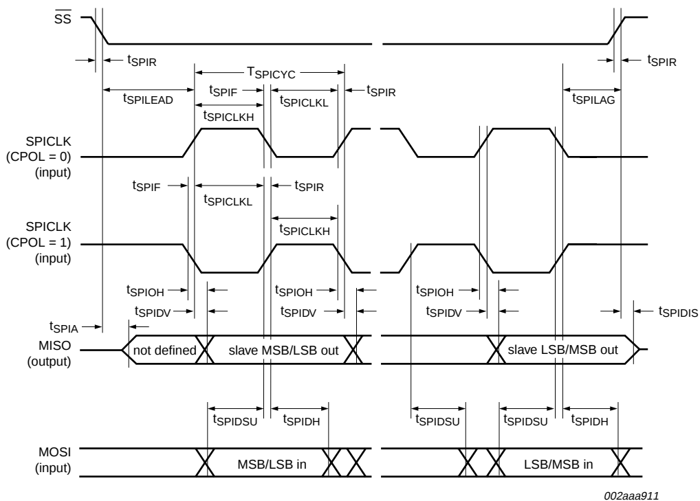
Fig 29. SPI slave timing (CPHA = 1)
