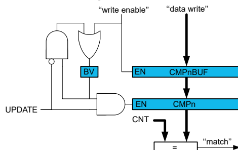
Figure 23-5. Period and Compare Double Buffering
