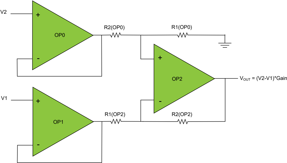
Figure 35-12. Instrumentation Amplifier
