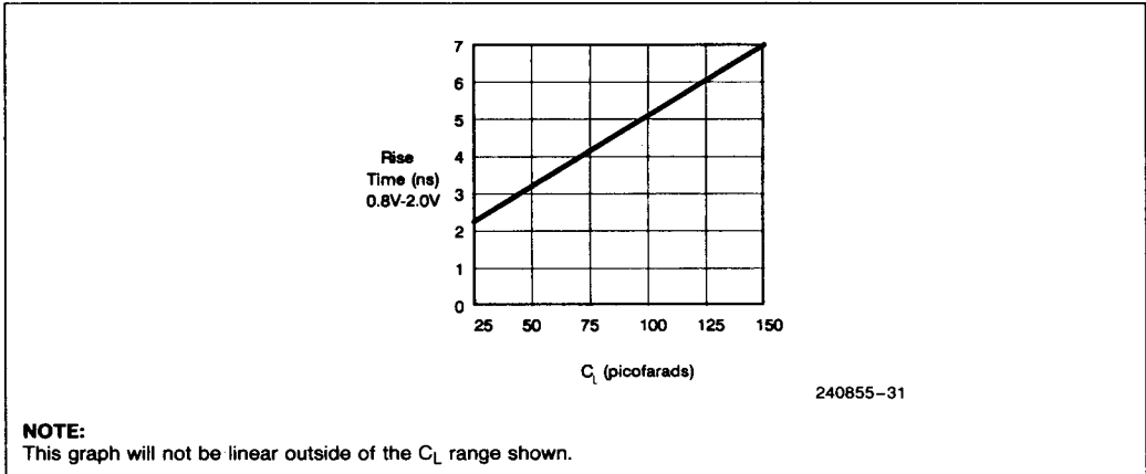
Figure 5-14. Typical Output Rise Time versus Load Capacitance under Worst Case Conditions
