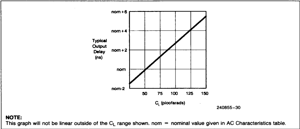
Figure 5-13. Typical Output Valid Delay versus Load Capacitance under Worst Case Conditions
