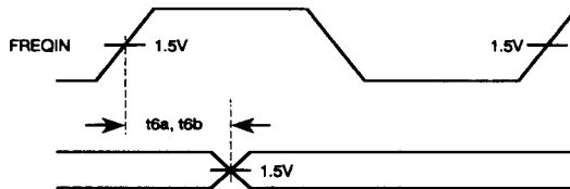
Figure 5-2. Output Waveforms
