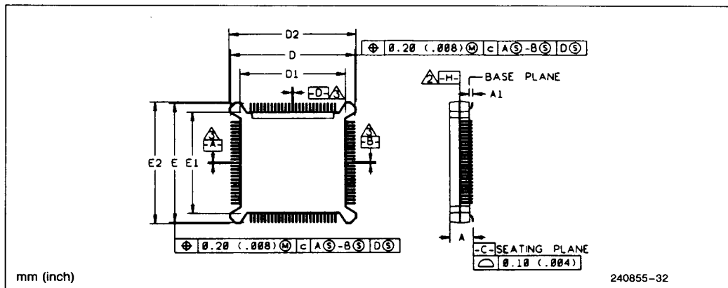
Figure 6-1. Principal Dimensions of the 82750DB in the 132-Lead PQFP Package
