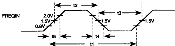
Figure 5-1. Clock Waveforms
