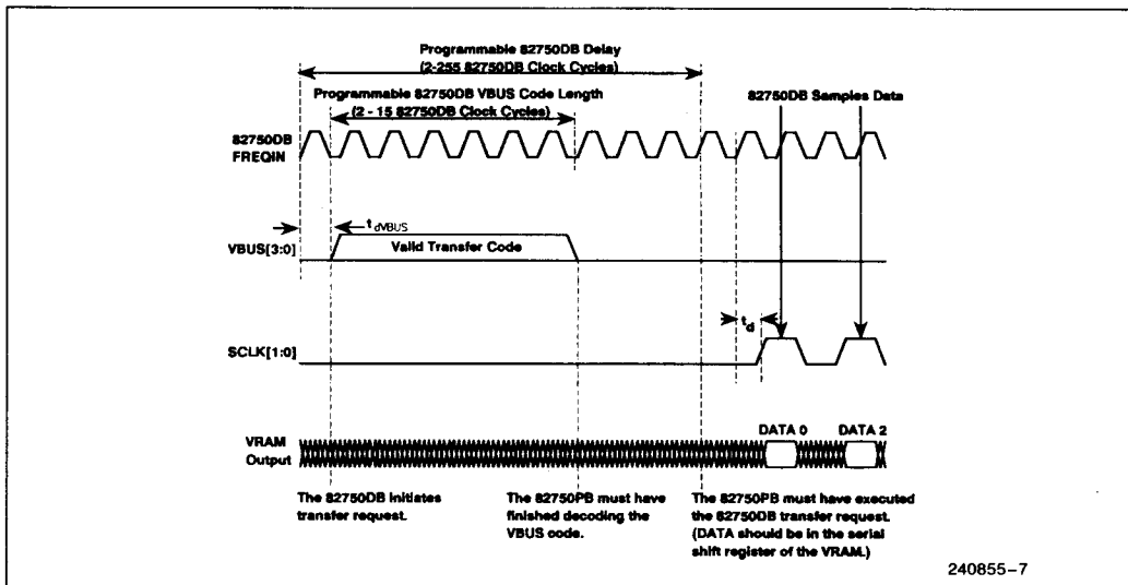
Figure 2-4. 82750PB/82750DB Communication
