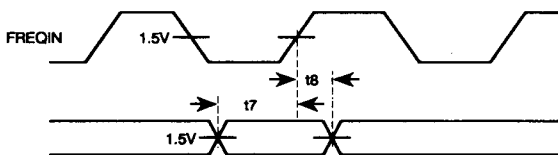
Figure 5-3. Input Waveforms
