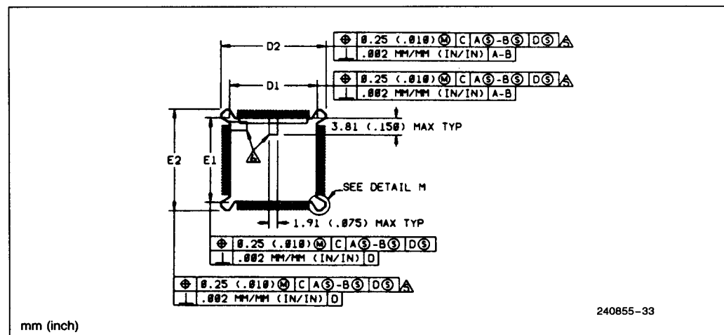
Figure 6-4. Detailed Dimensions of the 82750DB in the 132-Lead PQFP Package—Molded Details
