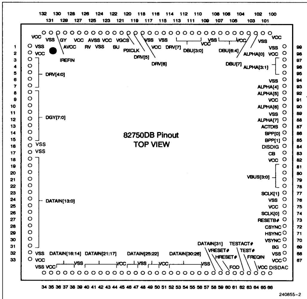
Figure 1-1. 82750DB Pinout
