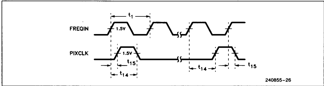
Figure 5-7. PIXCLK Waveforms
