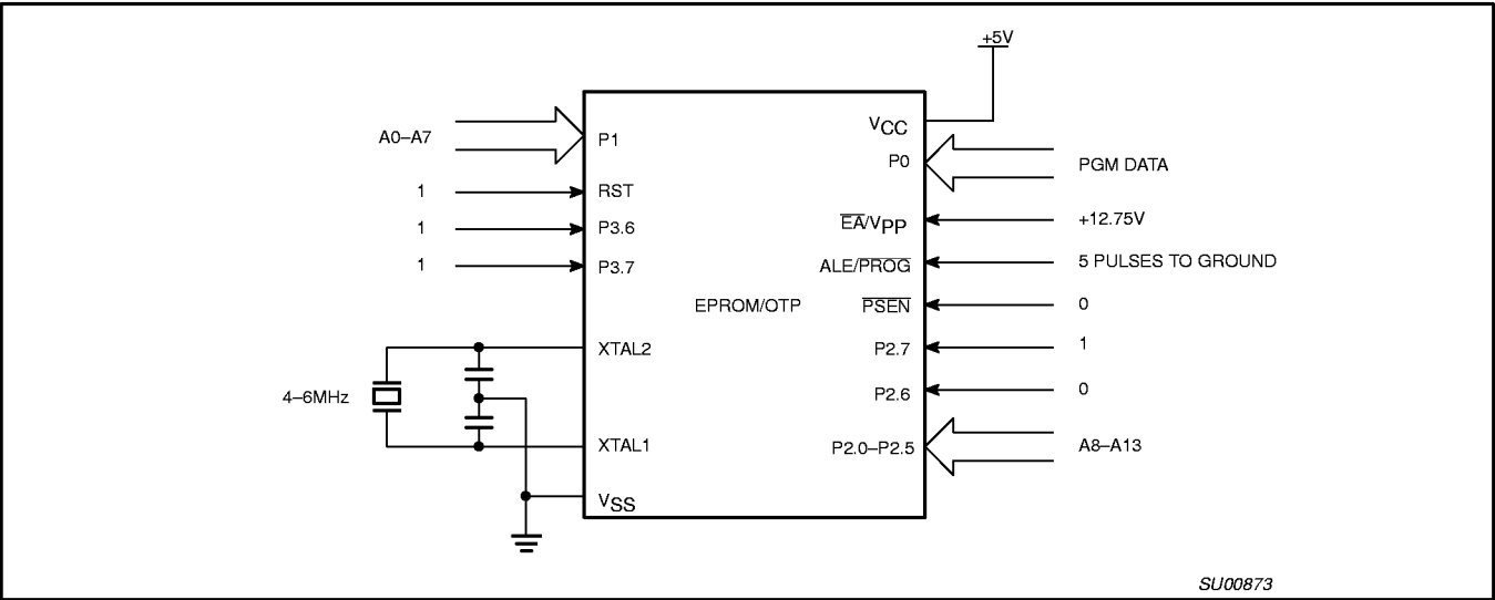
Figure 26. Programming Configuration
