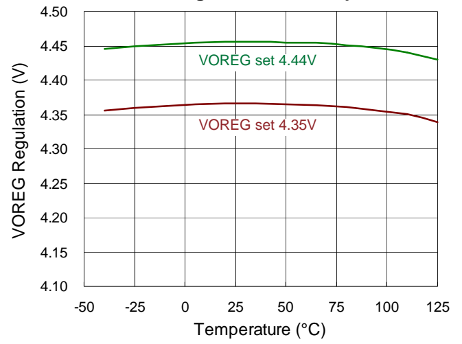
VOREG Regulation vs. Temperature
