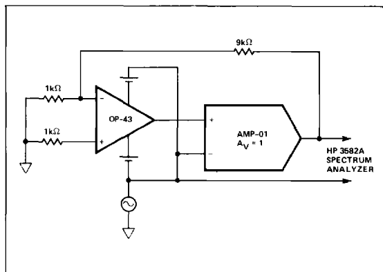
FIGURE 5: Circuit Used To Measure CMR From 10\text{Hz} to 29\text{kHz}
