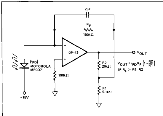
FIGURE 10: Photodetector/Fiber-Optic Receiver
