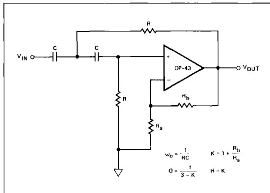
FIGURE 11: Highpass Filter
