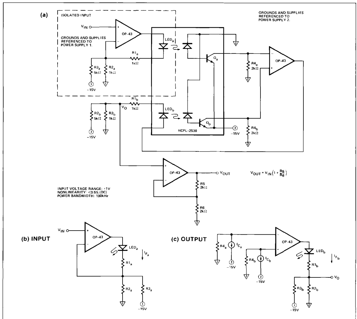
FIGURE 15: Isolation Amplifier
