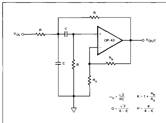
FIGURE 12: Bandpass Filter
