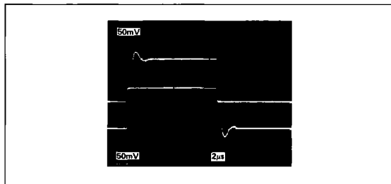
FIGURE 3: Small-Signal Transient Response at A_{VCL} = 5 with 1000\text{pF} Load
