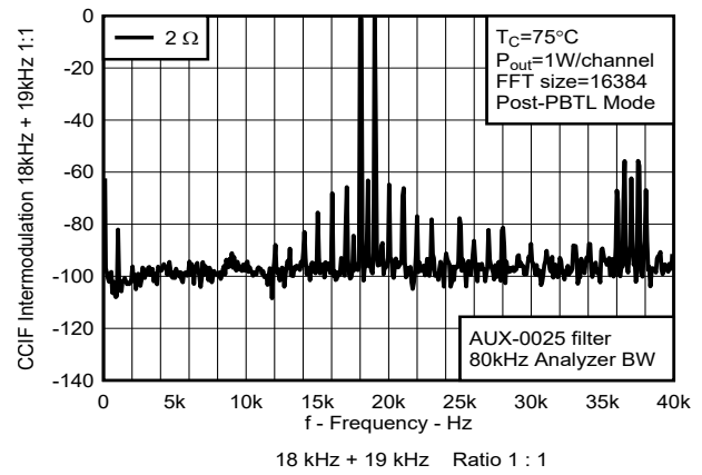
Figure 7-24. CCIF Intermodulation vs Frequency
