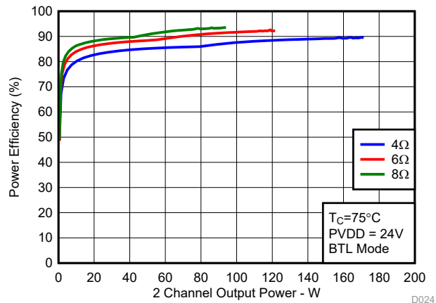
Figure 7-7. System Efficiency vs Output Power
