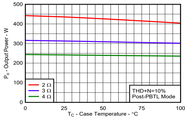
Figure 7-23. Output Power vs Case Temperature
