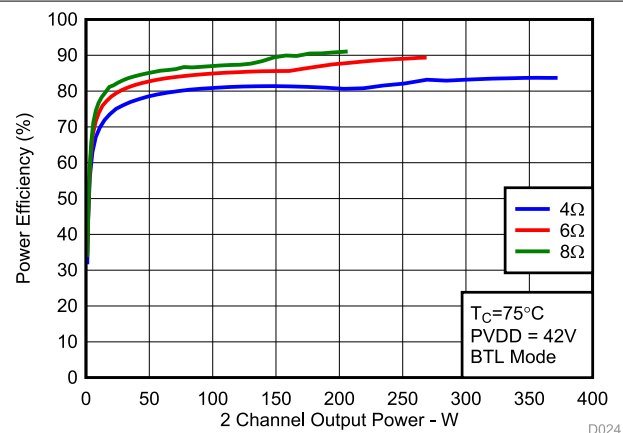
Figure 7-6. System Efficiency vs Output Power
