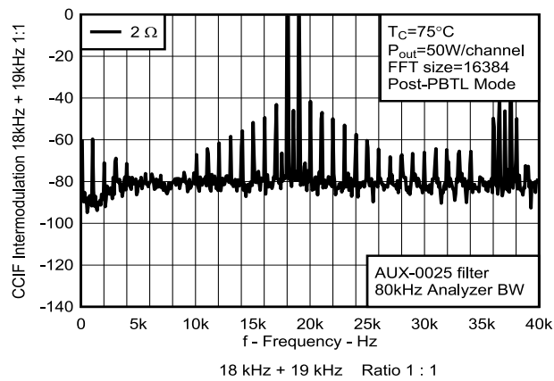
Figure 7-25. CCIF Intermodulation vs Frequency
