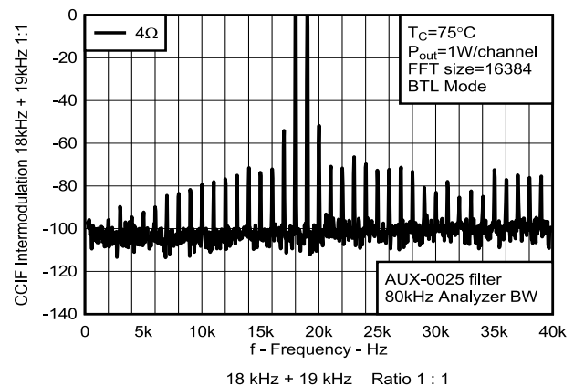
Figure 7-12. CCIF Intermodulation
