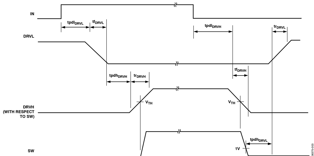
Figure 2. Timing Diagram
