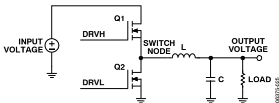
Figure 25. Buck Topology
