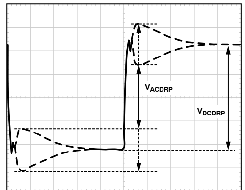
Figure 38. AC Load Line Waveform
