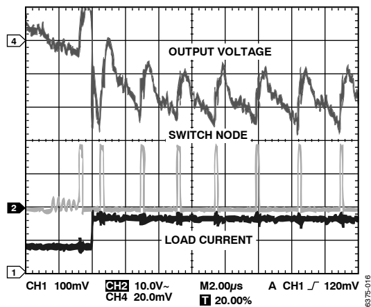
Figure 16. Load Transient, 2 A to 10 A, V_{IN} = 19 V
