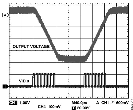
Figure 17. VID on the Fly, 1.25 V to 0.825 V
