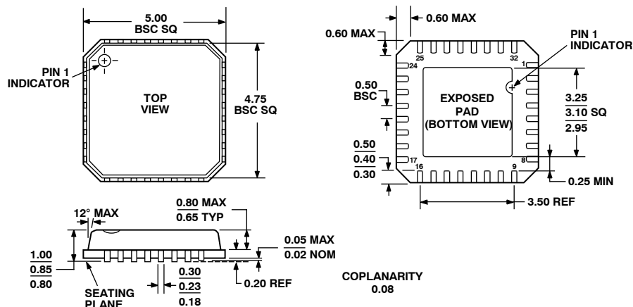
Figure 41. 32-Lead Lead Frame Chip Scale Package [LFCSP_VQ] 5 mm × 5 mm Body, Very Thin Quad (CP-32-2)
