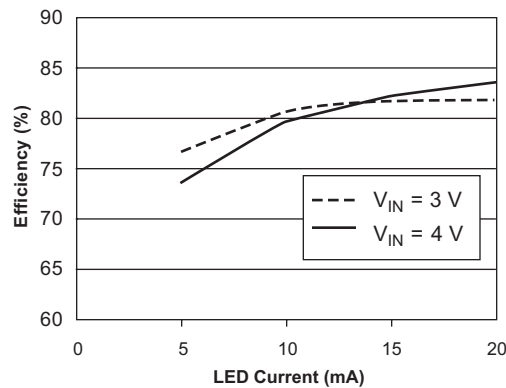
Conversion Efficiency versus Current
