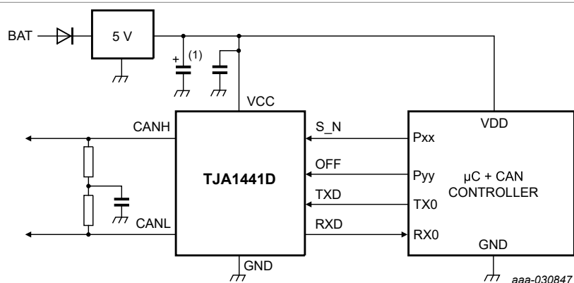
Figure 13. Typical TJA1441D application with a 5 V microcontroller
