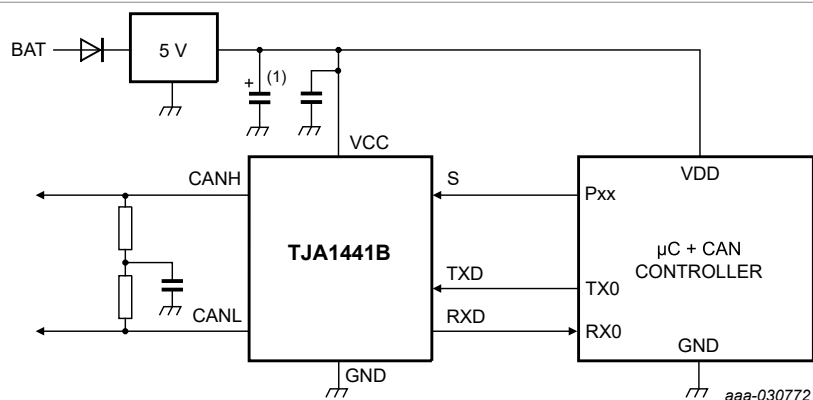
Figure 12. Typical TJA1441B application with a 5 V microcontroller
