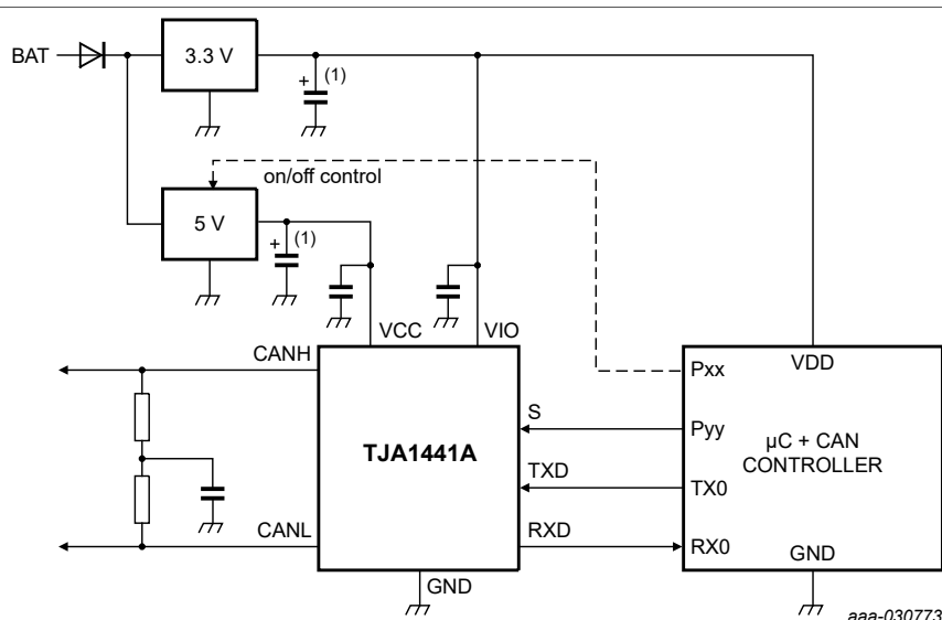
Figure 11. Typical TJA1441A application with a 3.3 V microcontroller
