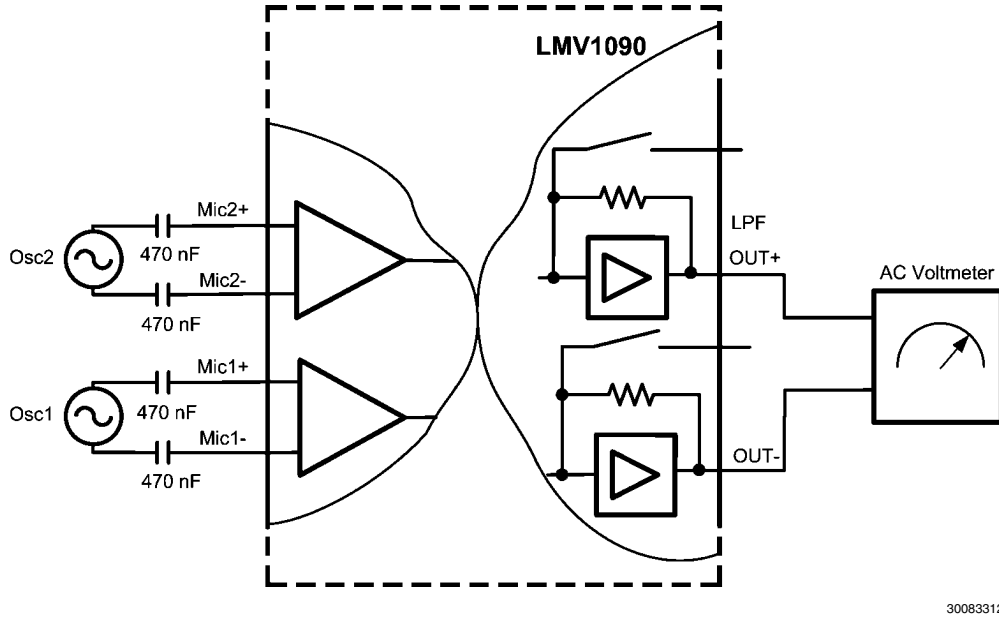
FIGURE 2. FFNS E , NFSL E , SNRI E Test Circuit
