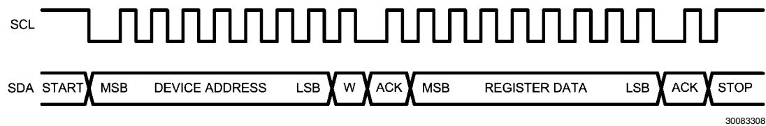
FIGURE 7. Start and Stop Diagram
