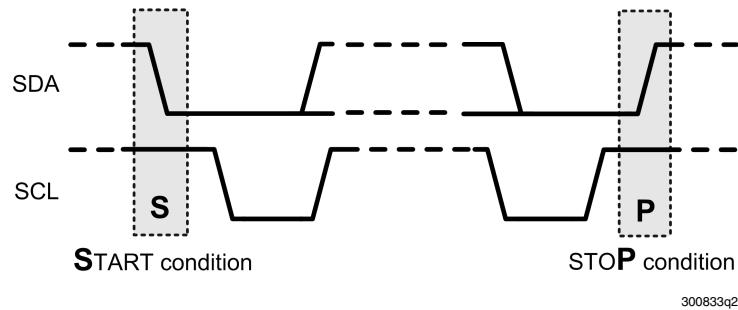
FIGURE 6. I 2 C Start Stop Conditions
