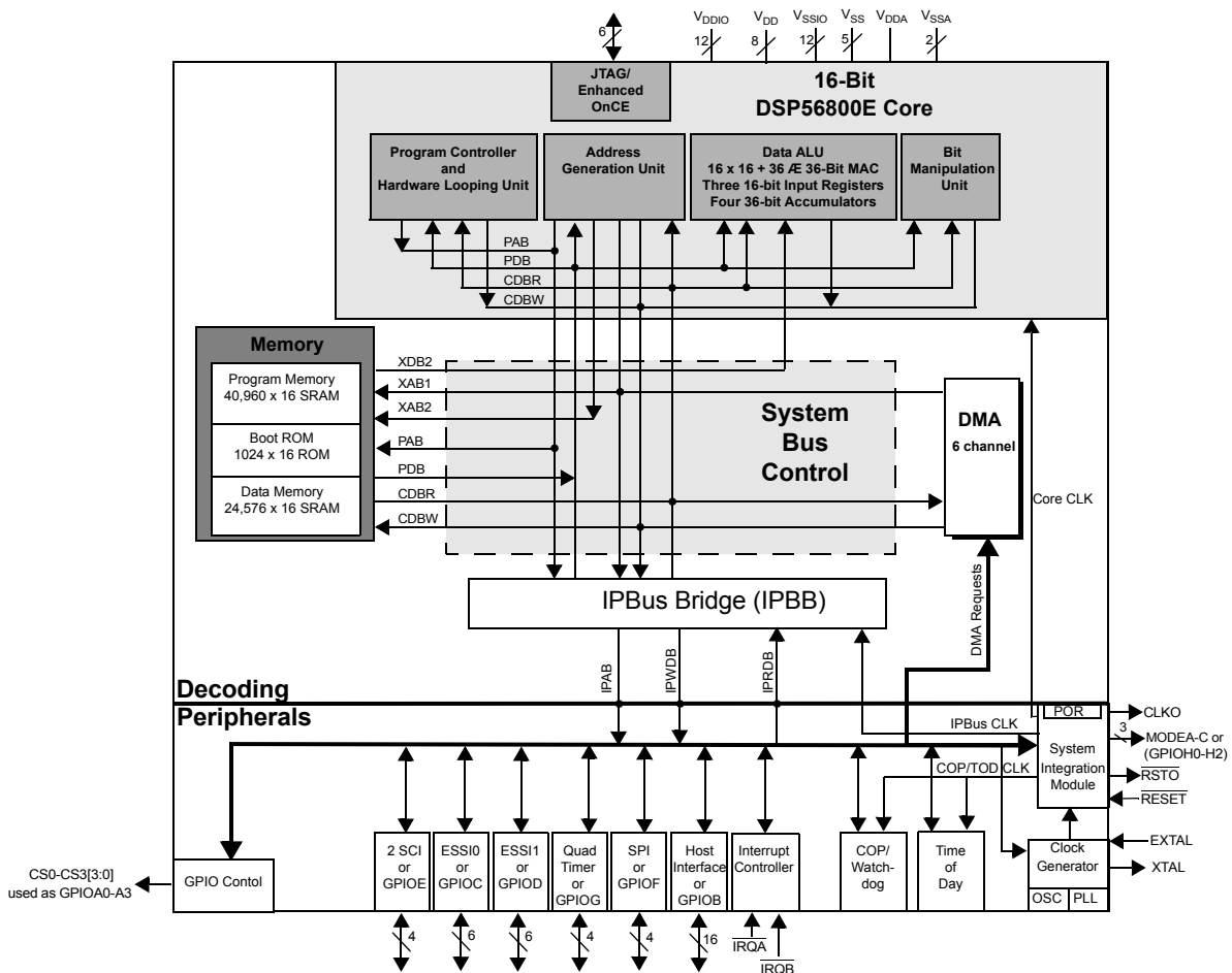
56857 Block Diagram
