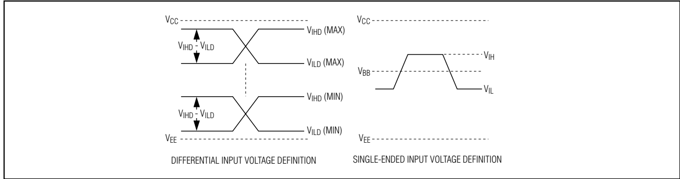
Figure 1. Input Definitions
