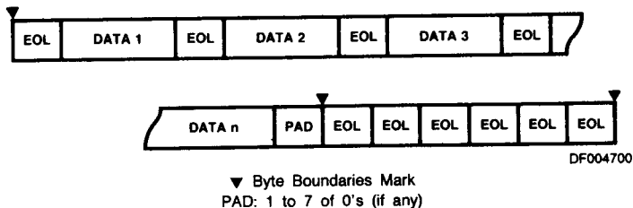
Figure 53. No Byte Boundary Conditioned with Auto EOL and No Time Fill
