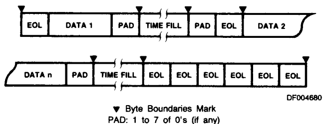
Figure 51. Byte Boundary Conditioned with Auto EOL and Time Fill
