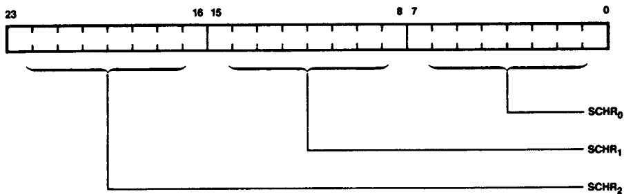
Figure 40. Source Count Holding Registers (CSCHR, ESCHR)
