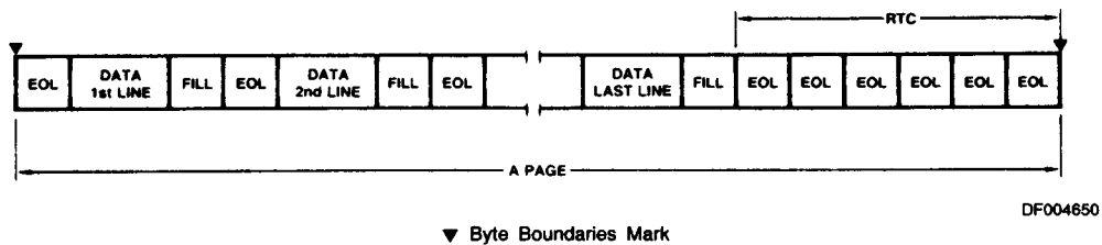
Figure 48. G-3 Compressed Data Format
