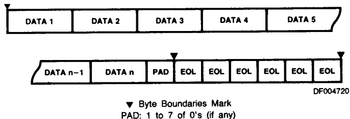
Figure 55. No Byte Boundary Conditioned without EOL and Time Fill
