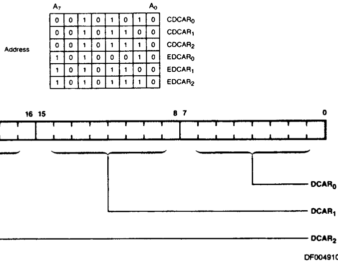
Figure 43. Destination Current Address Registers (CDCAR, EDCAR)
