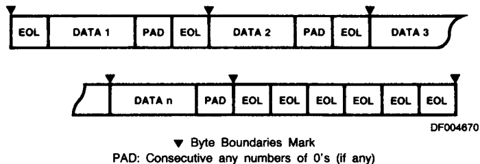
Figure 50. Byte Boundary Conditioned with Auto EOL and No Time Fill
