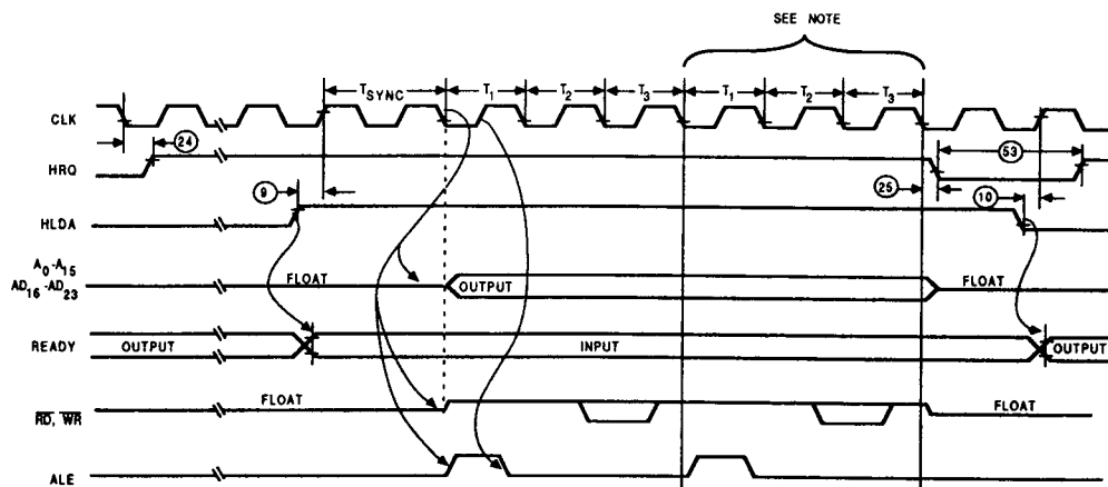
Timing Diagram 3. Bus Exchange Timing (System Interface)
