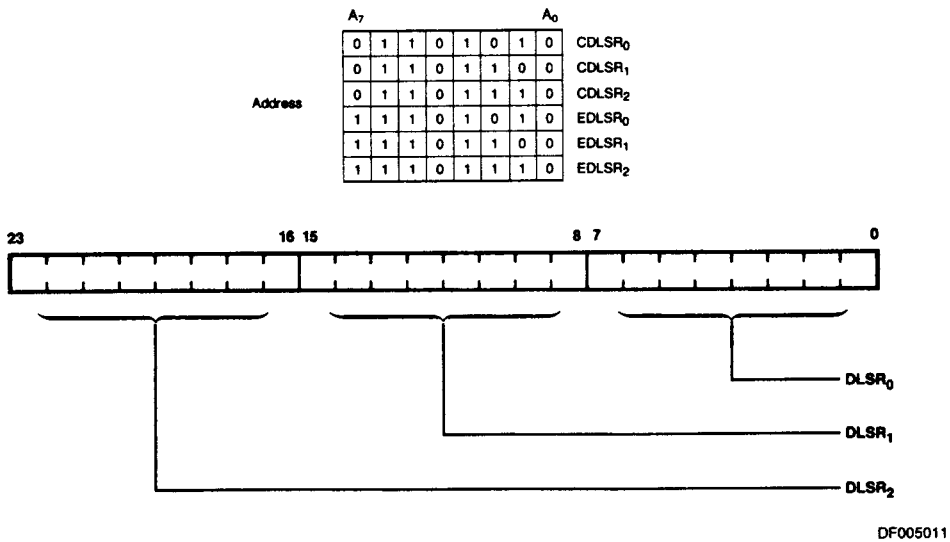
Figure 44. Destination Line Start Address Registers (CDLSR, EDLSR)
