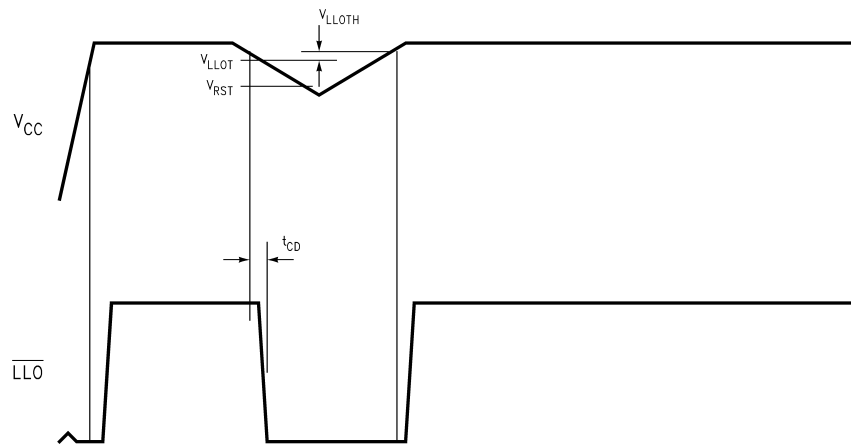
FIGURE 2. \overline{LLO} Output
