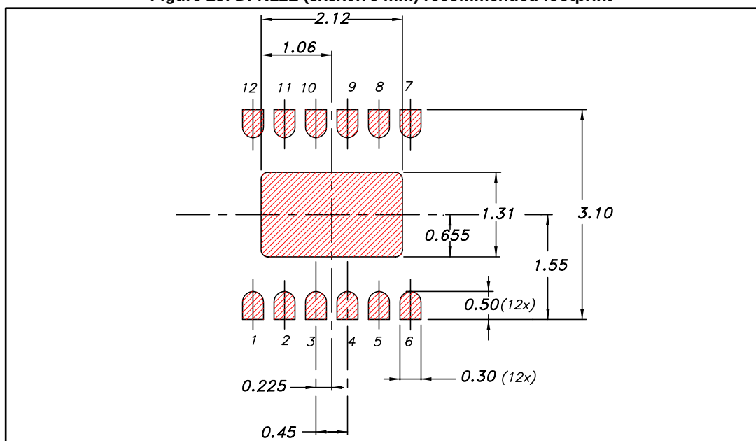
Figure 23: DFN12L (3x3x0.75 mm) recommended footprint
