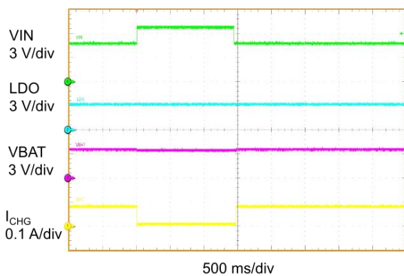
Figure 6: Input OVP
