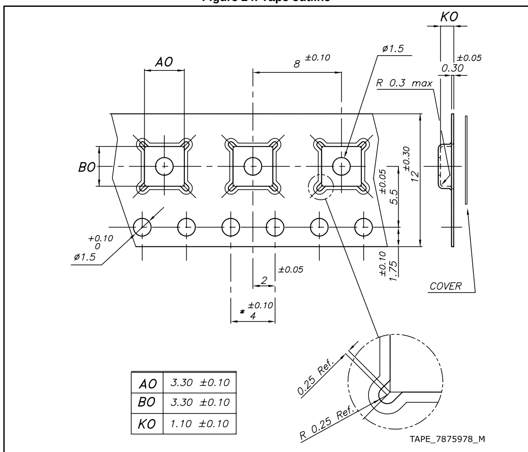
Figure 24: Tape outline
