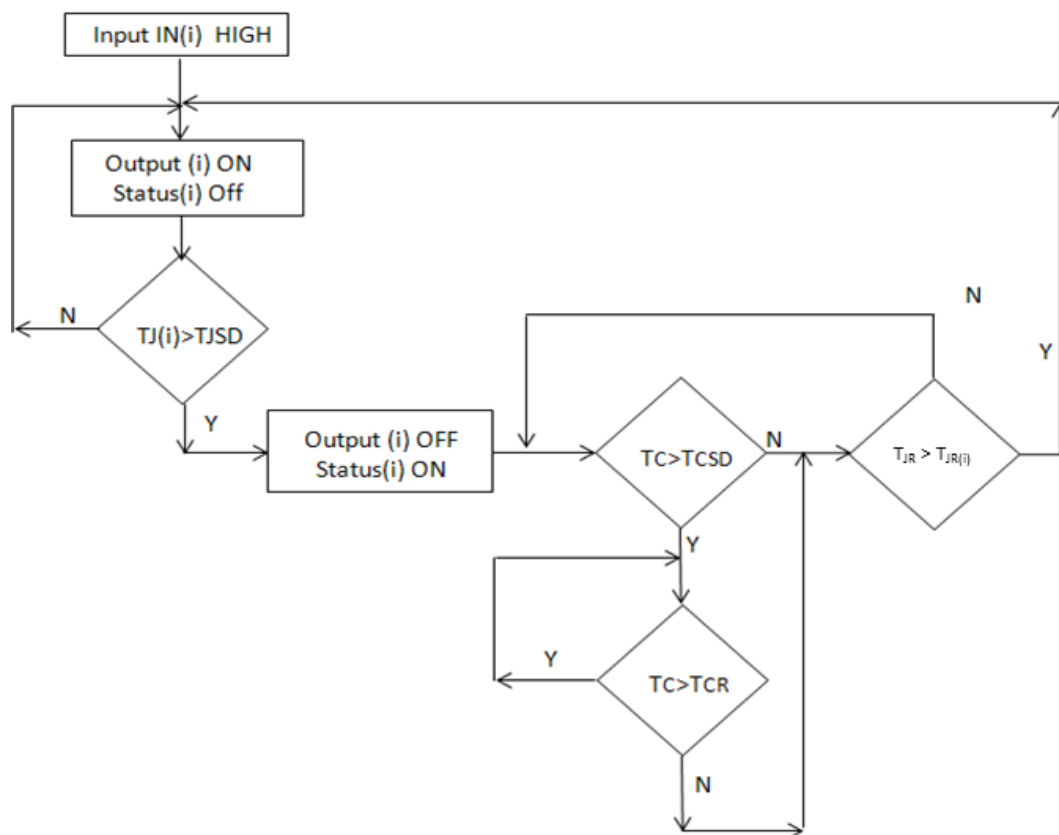
Figure 20. Thermal protection flowchart
