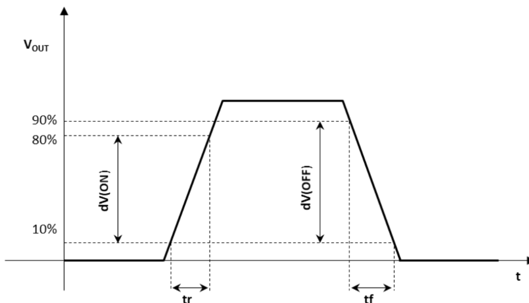
Figure 4. dV/dT definition
