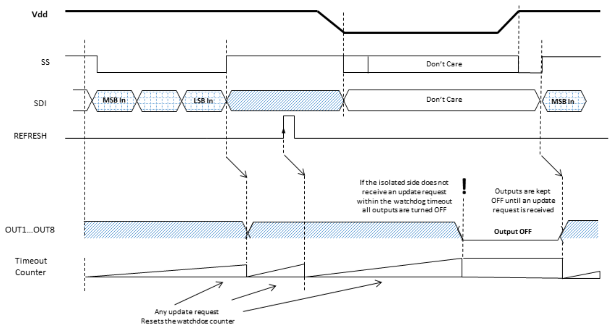
Figure 9. Watchdog behavior
