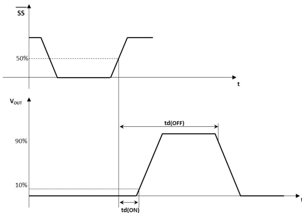
Figure 5. t_d(ON) - t_d(OFF) definition
