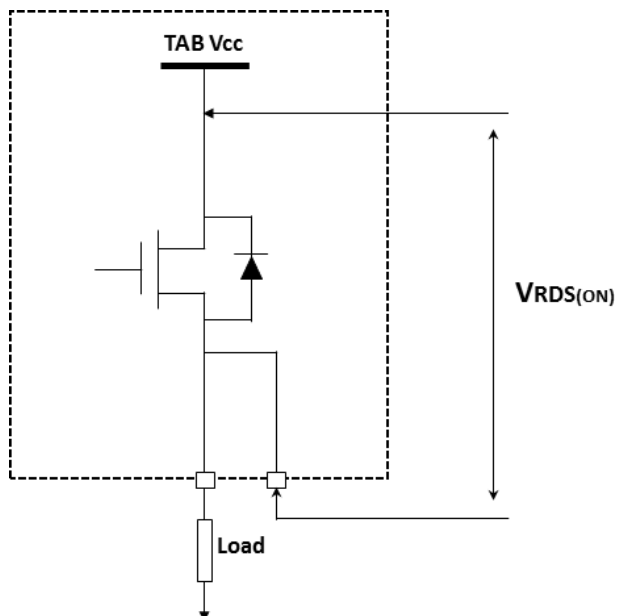
Figure 3. R_{DS(on)} measurement
