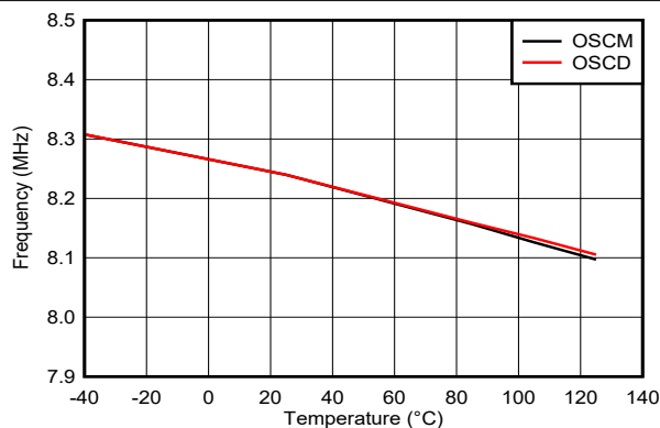
Figure 6-15. OSCM and OSCL Frequency vs Temperature
