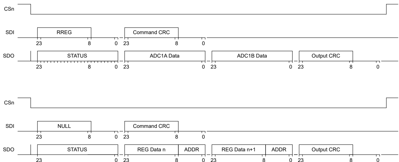
Figure 8-30. Bit Alignment, 24-Bit Word Size, RREG Command
