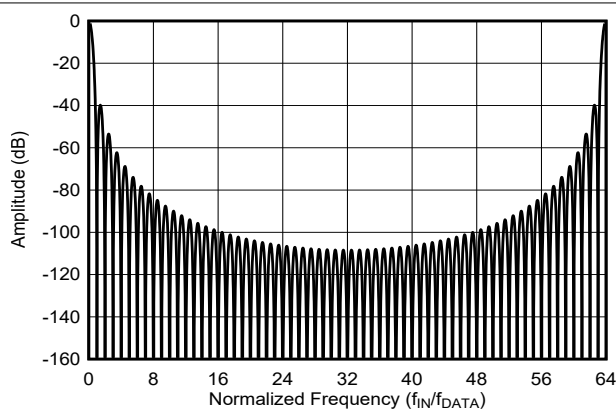
Figure 8-4. Sinc3 Filter Frequency Response to f_{MOD} (OSR = 64)
