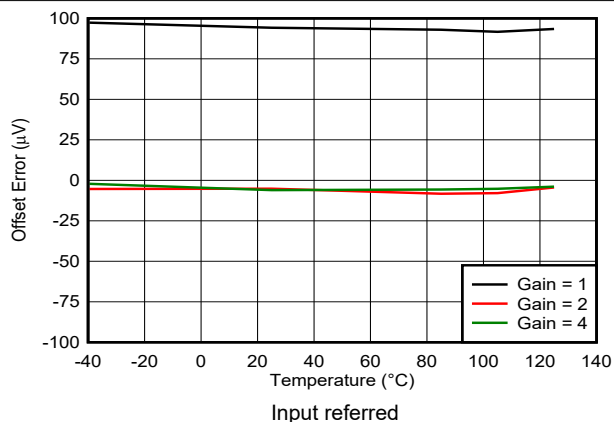
Figure 6-9. ADC2A Offset Error vs Temperature
