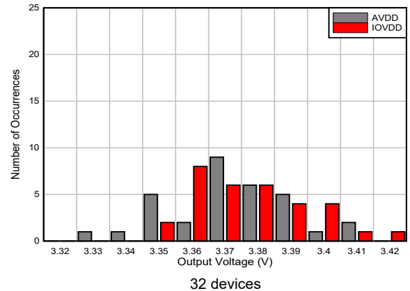
Figure 6-29. AVDD and IOVDD LDO Output Voltage Histogram
