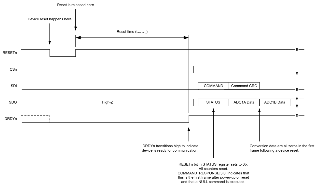
Figure 8-27. DRDYN Pin Behavior After Device Reset
