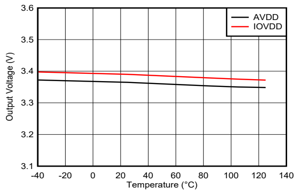
Figure 6-28. VCMA Output Voltage vs Temperature
