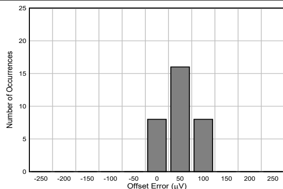
Figure 6-8. ADC2A Offset Error Histogram
