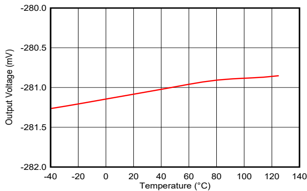
Figure 6-23. Test DACy Output Voltage vs Temperature
