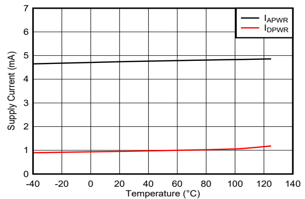
Figure 6-31. Supply Current vs Temperature Active mode, all ADCs enabled and converting
