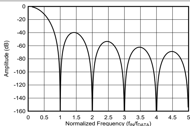
Figure 8-3. Sinc3 Filter Frequency Response
