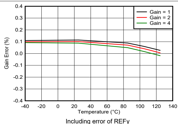
Figure 6-11. ADC2A Gain Error vs Temperature
