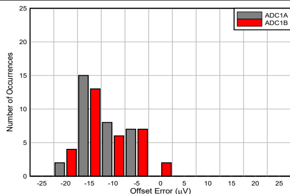
Figure 6-2. ADC1y Offset Error Histogram
