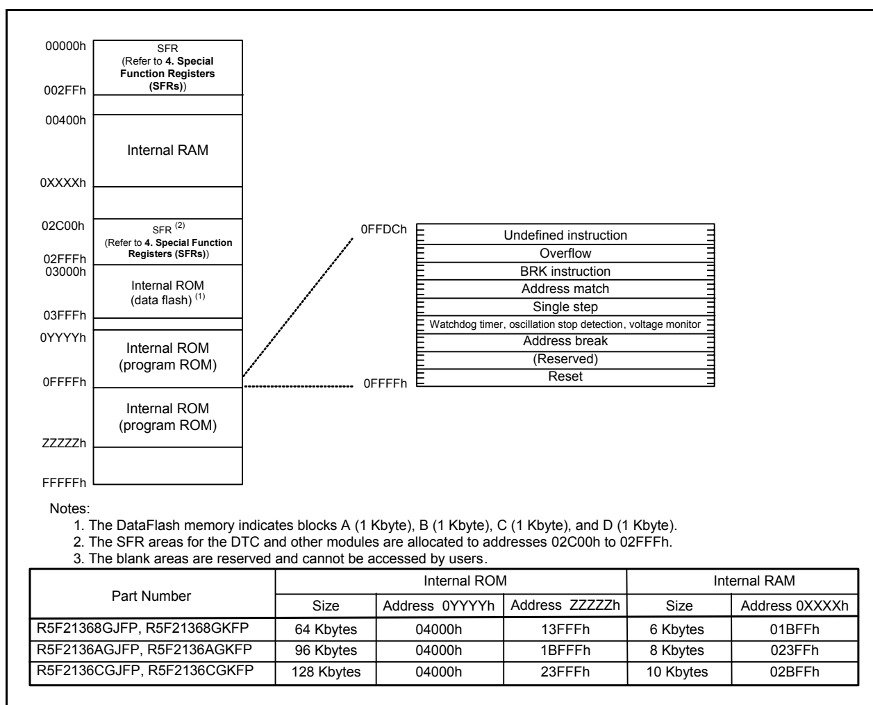
Figure 3.3 Memory Map of R8C/36G Group
