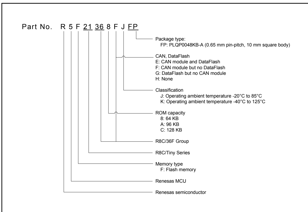
Figure 1.2 Part Number, Memory Size, and Package of R8C/36F Group
