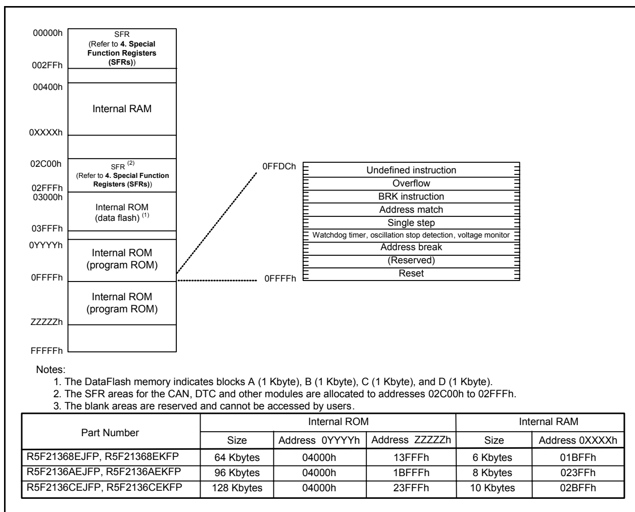
Figure 3.1 Memory Map of R8C/36E Group
