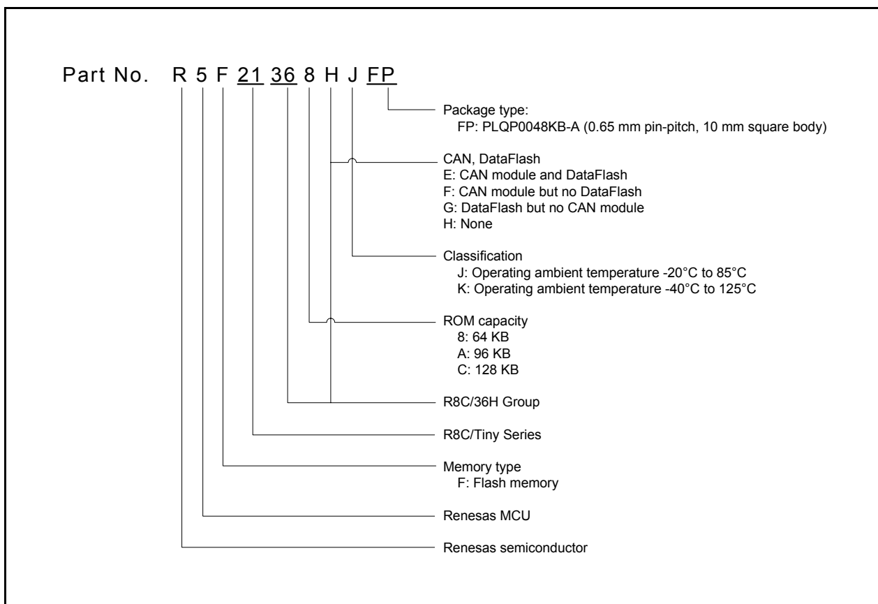
Figure 1.4 Part Number, Memory Size, and Package of R8C/36H Group
