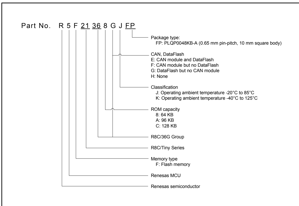
Figure 1.3 Part Number, Memory Size, and Package of R8C/36G Group
