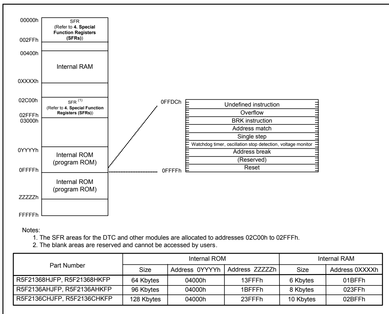
Figure 3.4 Memory Map of R8C/36H Group
