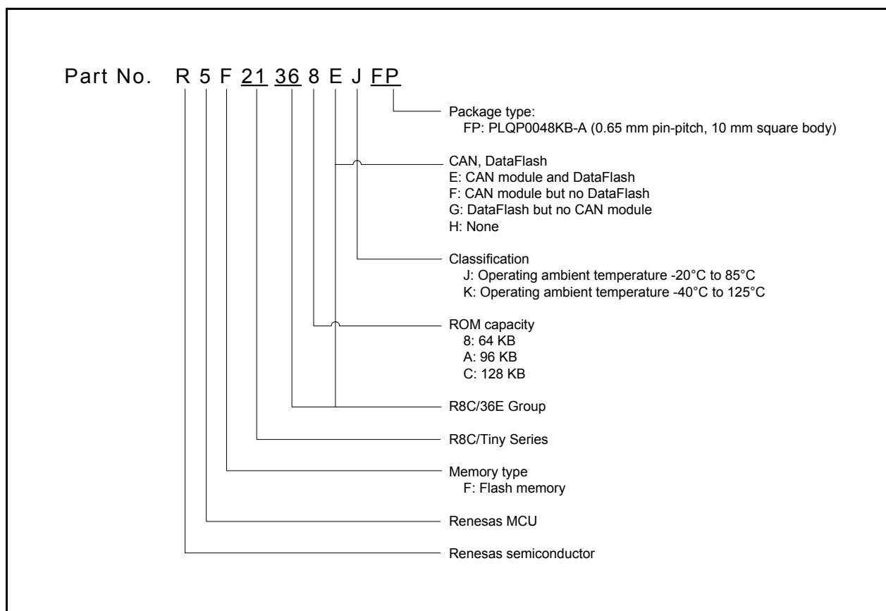
Figure 1.1 Part Number, Memory Size, and Package of R8C/36E Group
