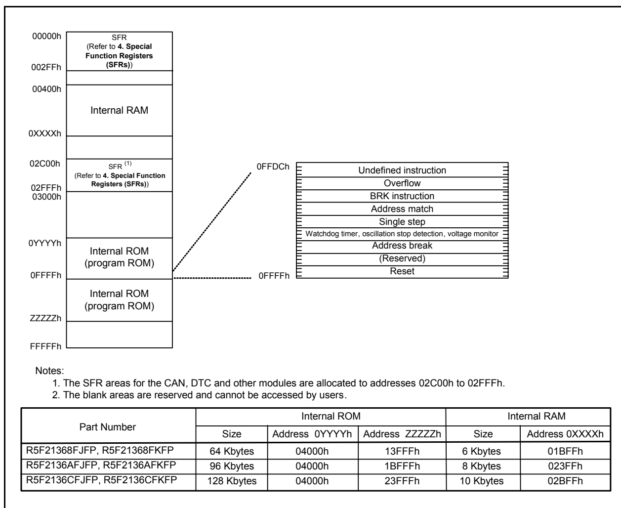
Figure 3.2 Memory Map of R8C/36F Group
