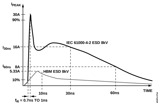
Figure 34. IEC 61000-4-2 ESD Waveform (8 kV) compared to the HBM ESD Waveform (8 kV)
