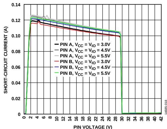
Figure 22. Short-Circuit Current vs. Pin Voltage
