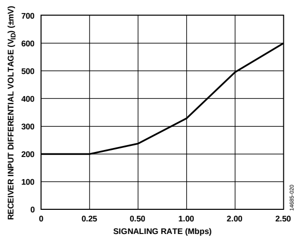
Figure 24. Receiver Input Differential Voltage ( V_{ID} ) vs. Signaling Rate
