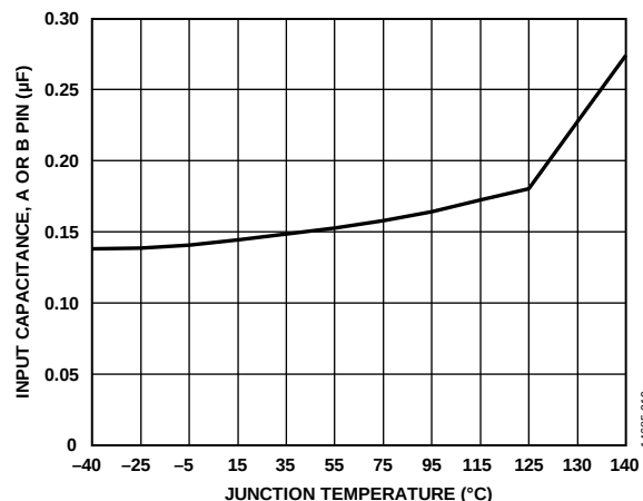
Figure 23. Input Capacitance, A or B Pin vs. Junction Temperature
