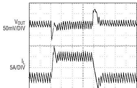
Transient Response
