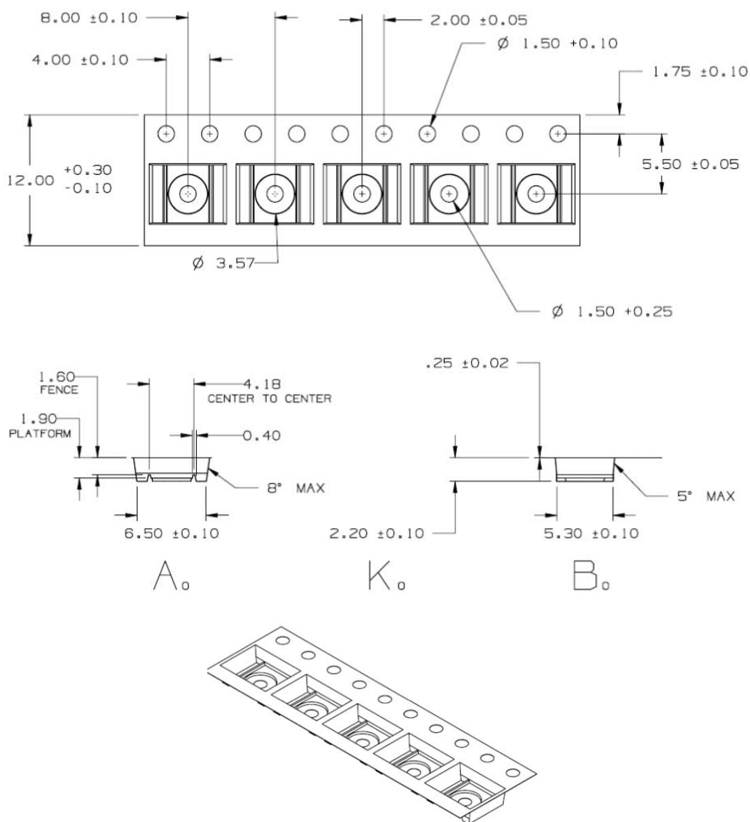
Figure 24. Power SO8 tape and reel
