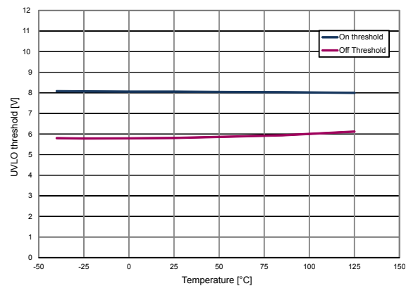
Figure 9. UVLO thresholds vs. temperature
