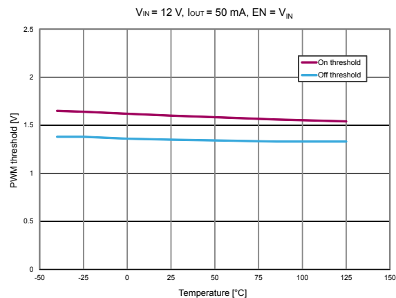
Figure 11. PWM thresholds vs. temperature
