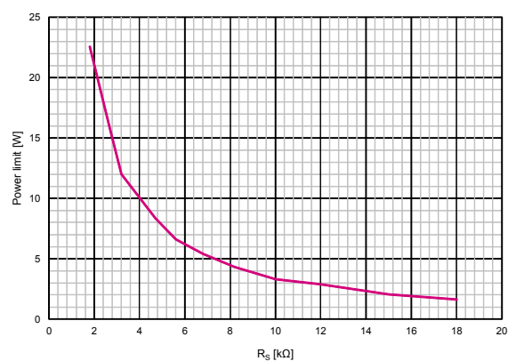
Figure 15. Power limit threshold vs. R_S
