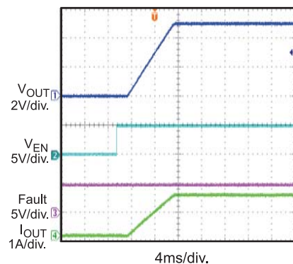
Start-Up through EN R_{LOAD} = 3.3\Omega
