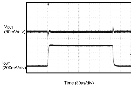
Figure 12. Load Transient ( V_{IN}=5V , V_{SET}=2V , V_{FON}=5V , C_{IN}=C_{OUT}=1\mu F , Slew Rate=250mA/μs)
