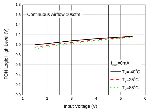
Figure 11. \overline{FON} Logic High Level vs. Input Voltage
