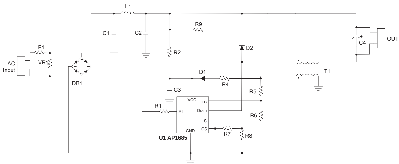
Typical Buck Application with Auxiliary Winding
