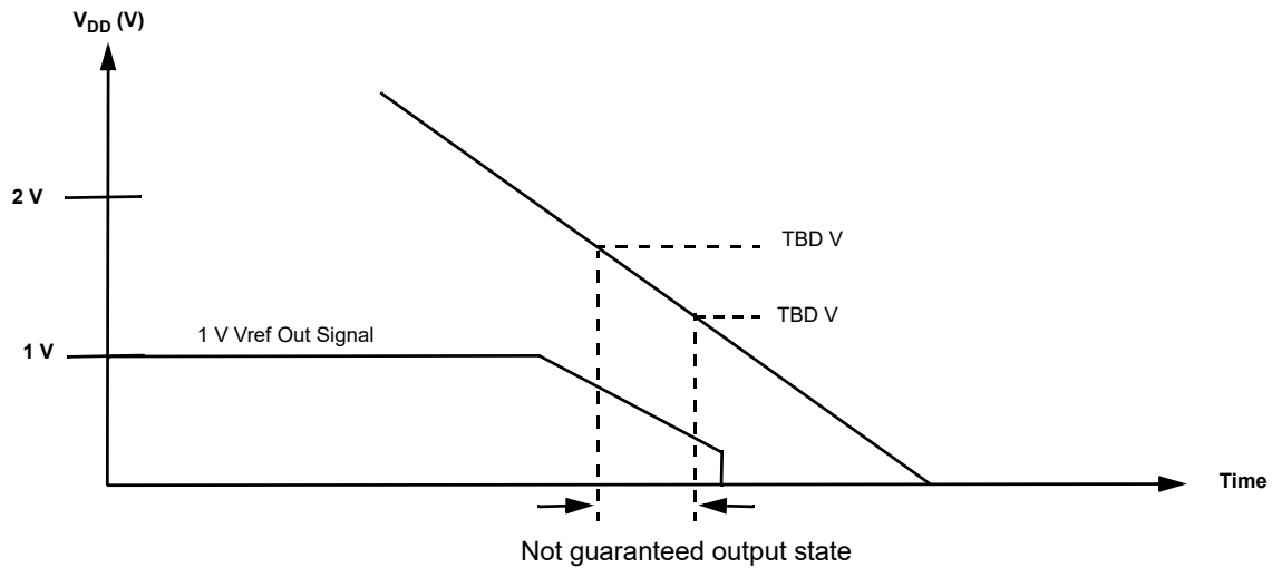
Figure 89: Power-Down
