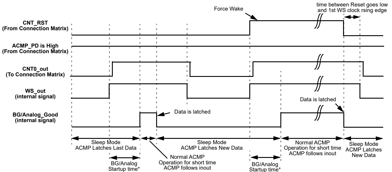
Figure 50: Wake/Sleep Timing Diagram, Normal Wake Mode, Counter Reset is Used
