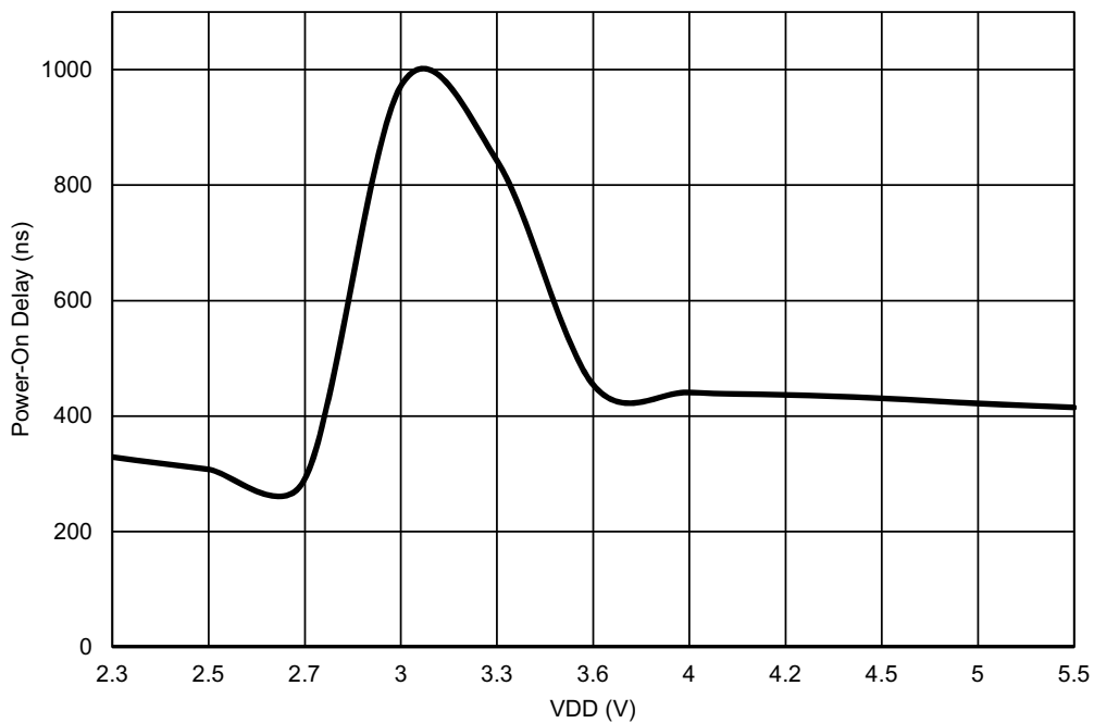
Figure 81: Oscillator1 Maximum Power-On Delay vs. V_{DD} at T = 25^\circ\text{C} , \text{OSC1} = 2.048\text{ MHz}
