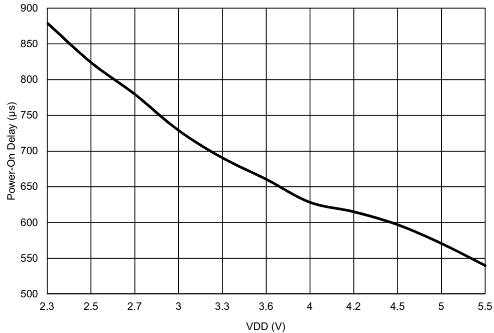
Figure 80: Oscillator0 Maximum Power-On Delay vs. V_{DD} at T = 25^\circ\text{C} , \text{OSC0} = 2.048\text{ kHz}
