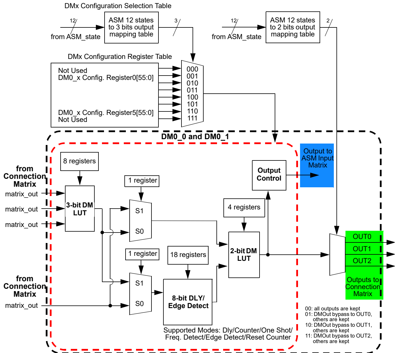
Figure 117: DM0_0/DM0_1 Outputs
