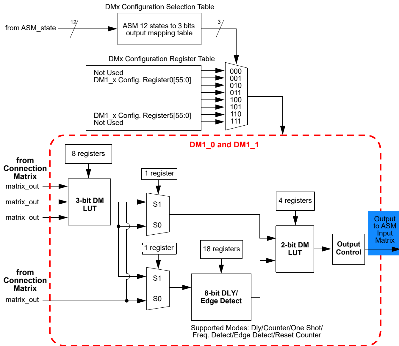
Figure 118: DM1_0/DM1_1 Outputs
