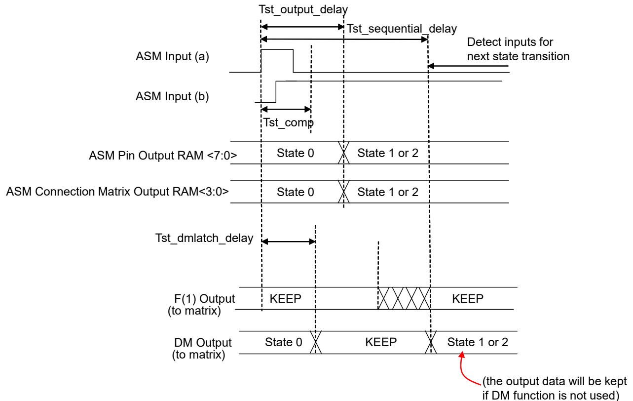
Figure 102: State Transition - Competing Inputs
