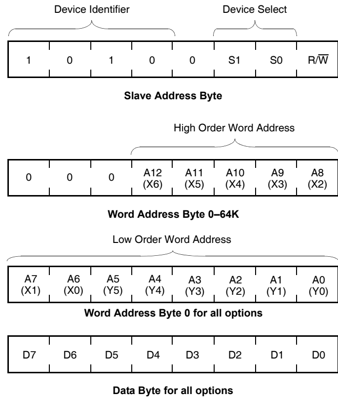
Figure 15. X4643/5 Addressing
