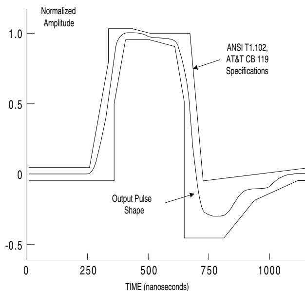
Figure 6. Pulse Mask at T1/J1 Interface
