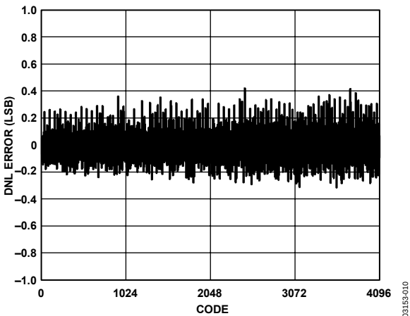
Figure 10. Typical DNL for the AD7451 for V DD = 5 V
