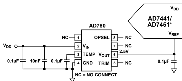
Figure 27. Typical V_{\text{REF}} Connection Diagram for V_{\text{DD}} = 5 V
