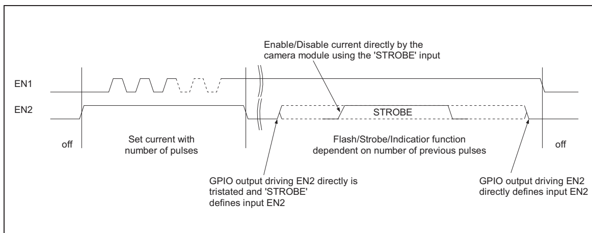
Figure 35: AS3685B Example Two Wire Interface Driving Waveform
