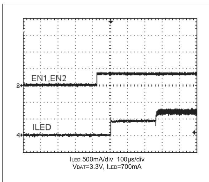
Figure 18: Startup of AS3685A -- I_{LED} Current
