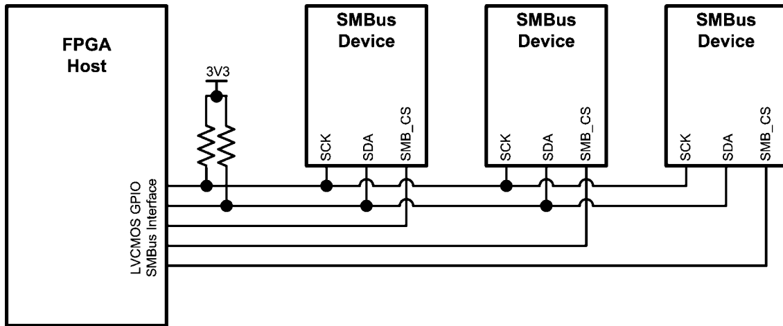
FIGURE 9. SMBus Configuration 2
