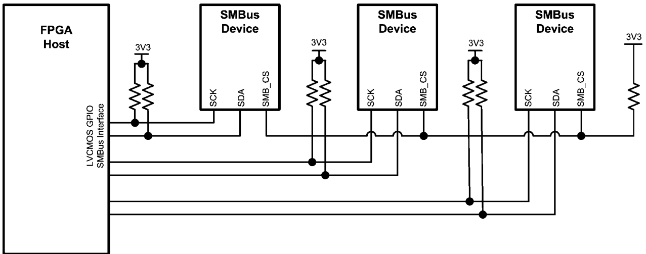
FIGURE 10. SMBus Configuration 3
