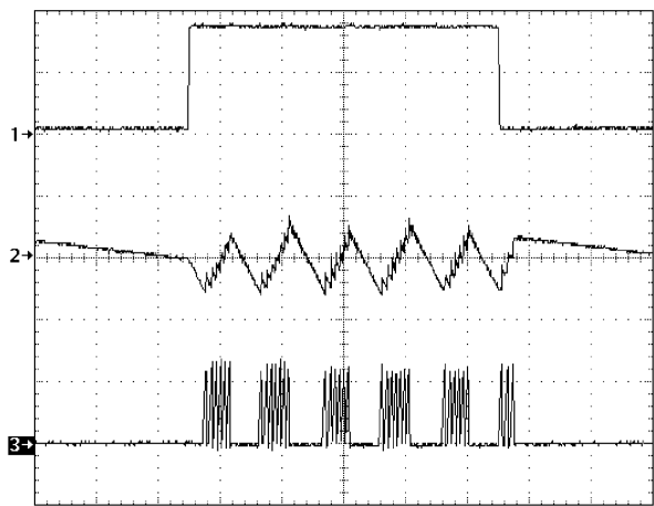
Step Response
