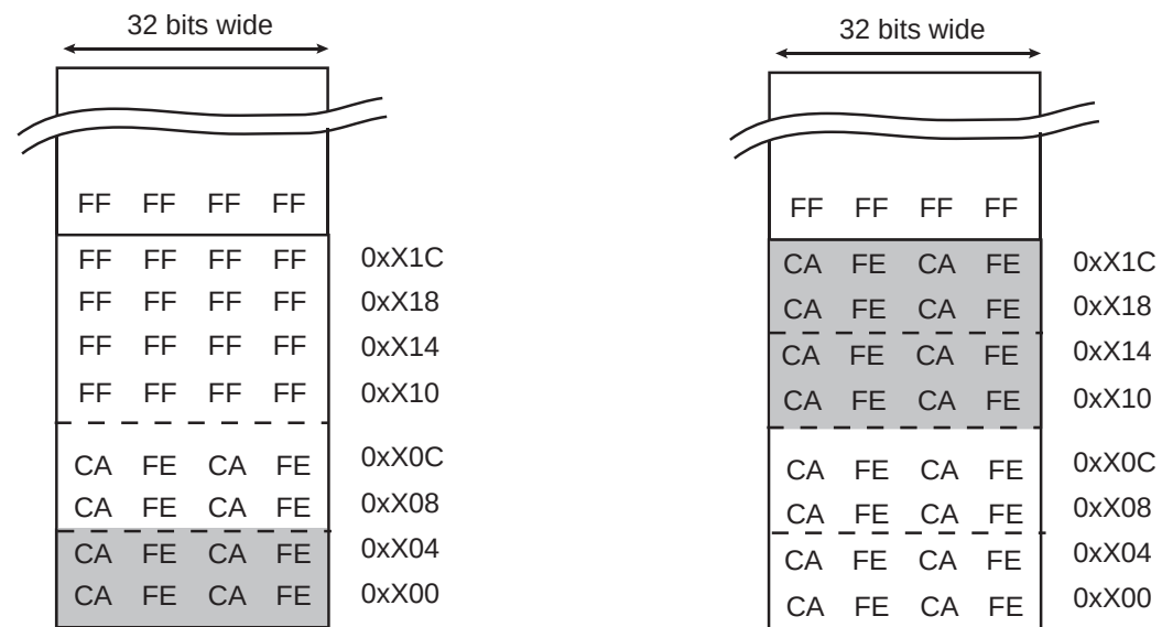
Step 3: Flash array after programming a second 64-bit data at address 0xX00 (write latch buffer + WP)
