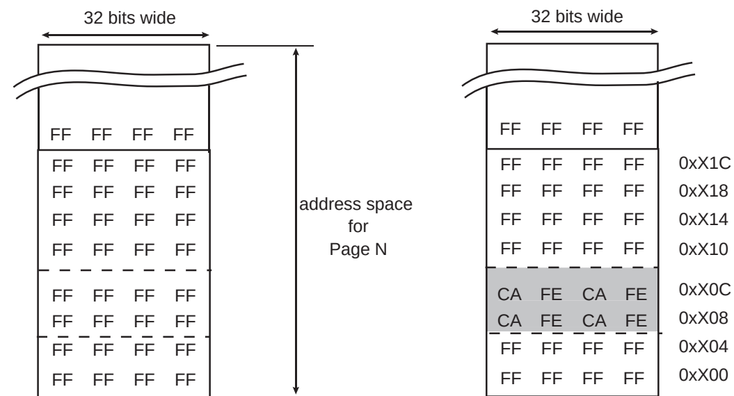
Step 1: Flash array after page erase
