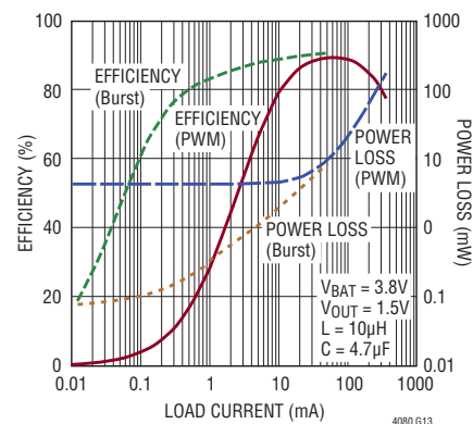
Buck Efficiency vs Load Current ( V_{OUT} = 1.5V )
