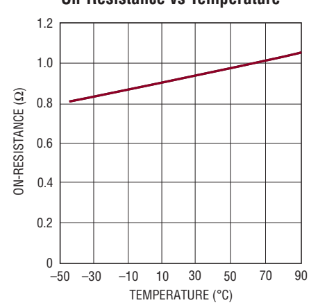
Buck Main Switch (PMOS) On-Resistance vs Temperature
