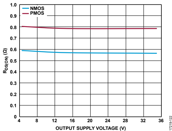
Figure 29. Output Resistance ( R_{DS(ON)} ) vs. Output Supply Voltage for NMOS and PMOS, V_{DD1} = 5\text{ V}
