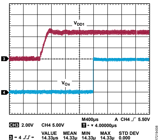
Figure 15. Typical V_{DD1} Delay to Output Waveform, V_{ix} = V_{DD1} and PWM = V_{DD1} or GND_1
