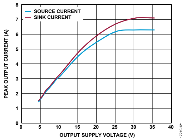
Figure 28. Peak Output Current vs. Output Supply Voltage with a 2.2\text{ }\Omega Series Gain Resistor
