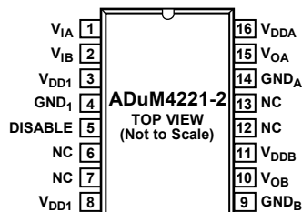
Figure 7. ADuM4221-2 Pin Configuration
