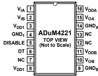
Figure 5. ADuM4221 Pin Configuration
