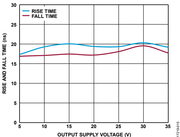
Figure 22. Rise and Fall Time vs. Output Supply Voltage with a 3.9Ω Series Gate Resistor for a 2 nF Load
