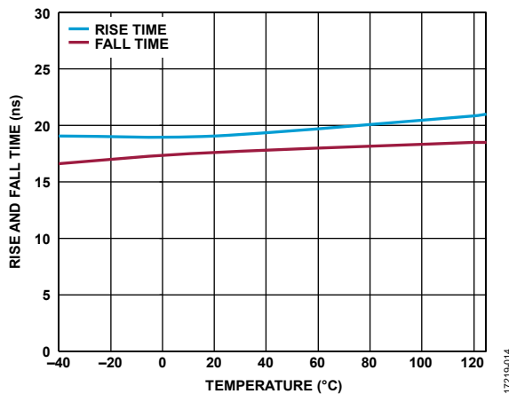
Figure 21. Rise and Fall Time vs. Temperature with a 3.9Ω Series Gate Resistor for a 2 nF Load and a 15 V Output Supply
