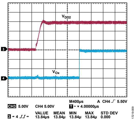
Figure 16. Typical V_{DD2} Delay to Output Waveform, V_{ix} = V_{DD1} and PWM = V_{DD1} or GND_1 ( V_{DD2} Refers to V_{DDA} or V_{DDB} )
