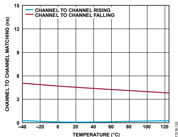
Figure 27. Channel to Channel Matching vs. Temperature, Rising and Falling, V_{DD2} = 15\text{ V} ( V_{DD2} Refers to V_{DDA} or V_{DDB} )
