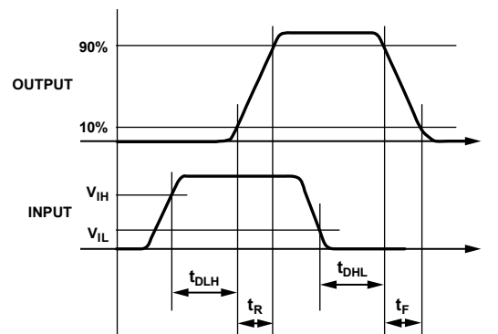
Figure 33. Propagation Delay Parameters
