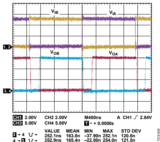
Figure 10. Dead Time Operation Between Input and Output with 50 kΩ Dead Time Resistor (ADuM4221 Only)
