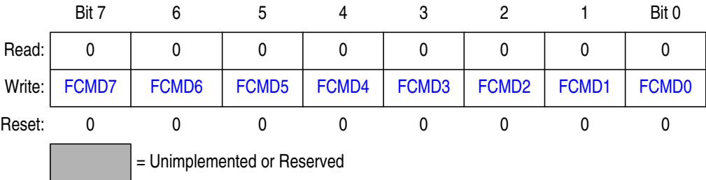
Figure 4-9 FLASH Command Register (FCMD)
