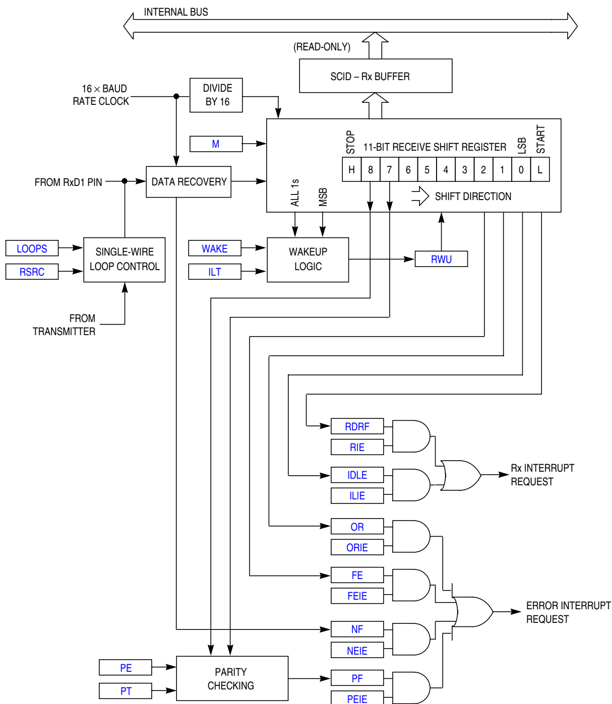
Figure 11-4 SCI Receiver Block Diagram
